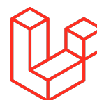
Laravel
