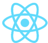
React Native
